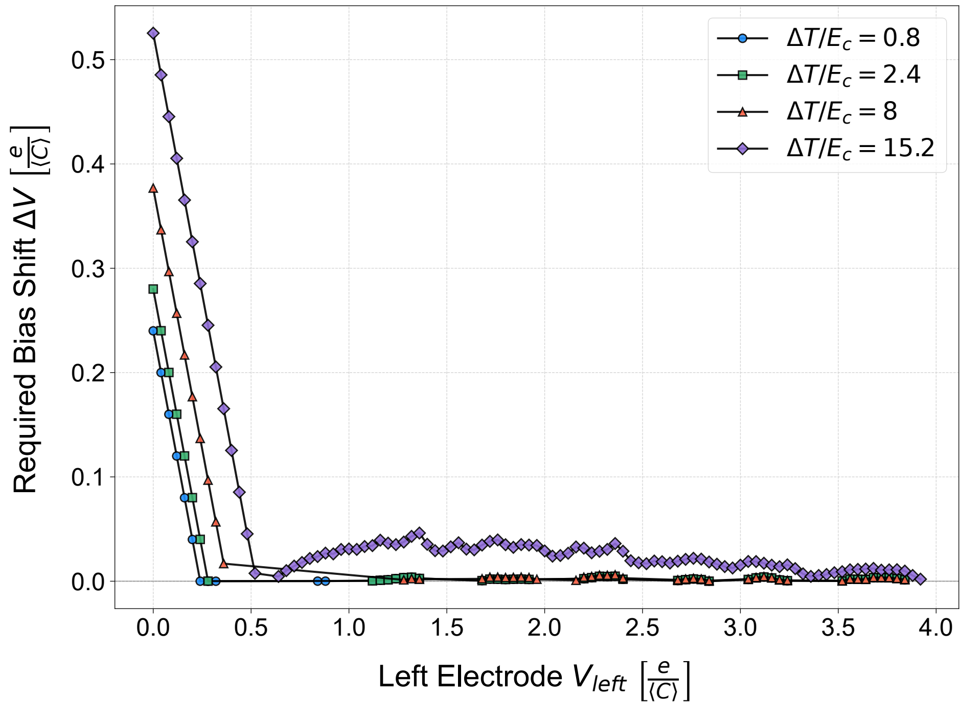
Counteracting Bias \Delta V to Maintain I(V_{left}, \Delta T = 0)
